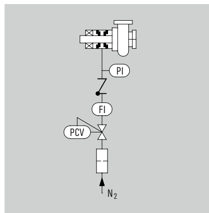
Operating and installation diagram for a GSS system.
