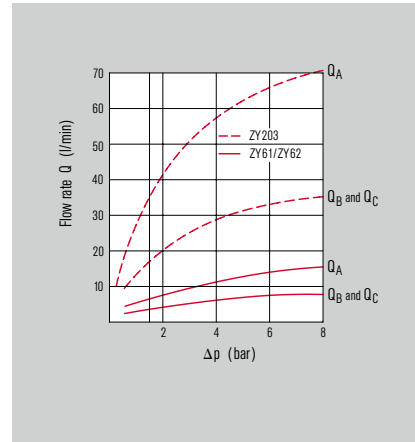
Flow rates for water as medium.
