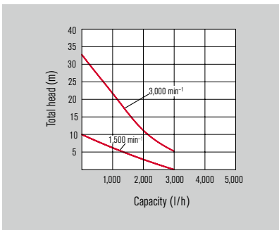
Pumping characteristic with water as medium
