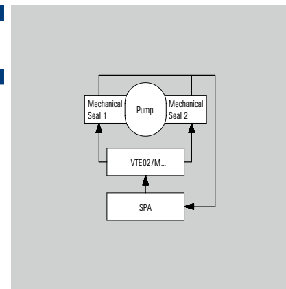
Operating diagram for the VTE02/M...
