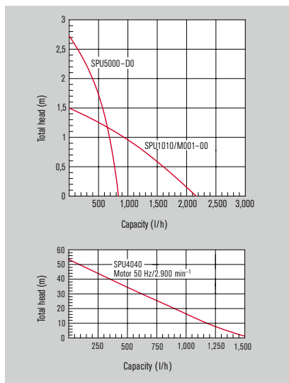
Pumping characteristic for media with viscosity < 15 cSt
