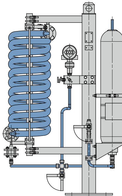
SPB6002-A4 with Air cooler
