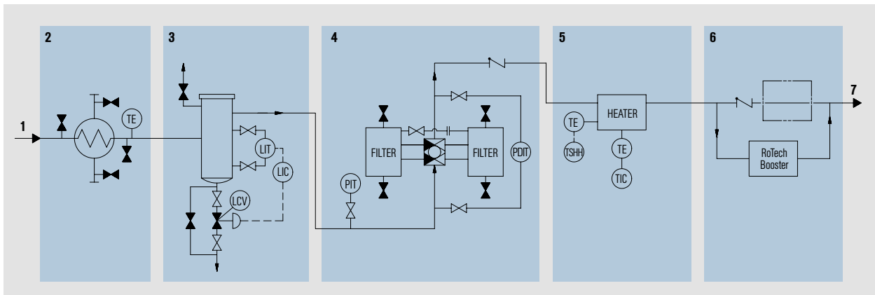
Example of a gas conditioning system (skid).
