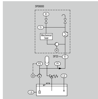
Operating and installation diagram for an automatic refill unit.
