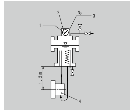
Operating and installation diagram for a TS3016 system
