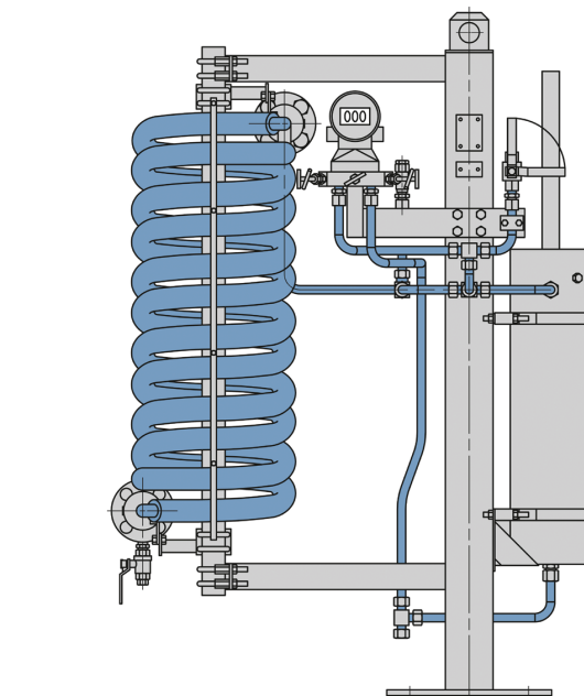
SPC6002-A4 with air cooler
