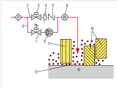
Operating and installation diagram for a RoTechBooster
