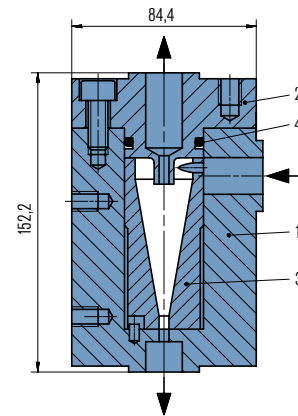
ZY61 in block-type design with integrated flange
