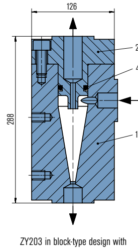
ZY203 in block-type design with integrated flange
